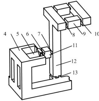
Fig. 1. (b) The kinematic chain schematic
