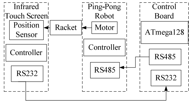
Fig. 3. Hardware of control system
