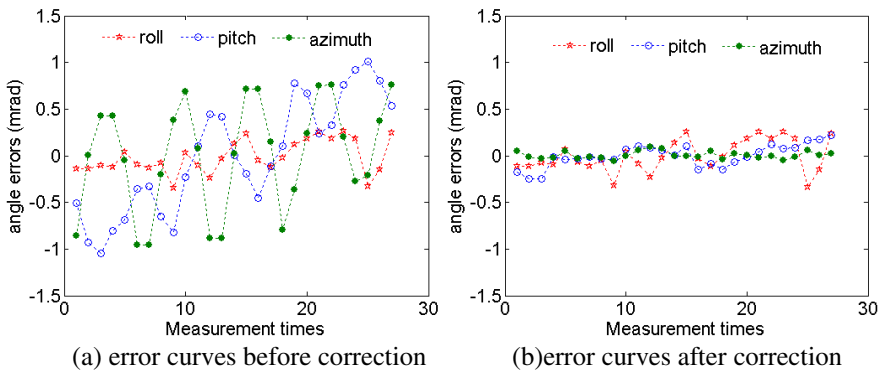
Fig. 6. The error curves of attitude angles in repeated experiment
