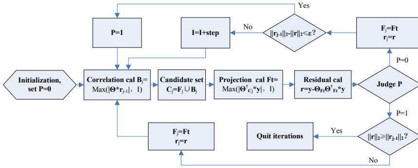
Fig. 1. FSAMP algorithm flow chart
