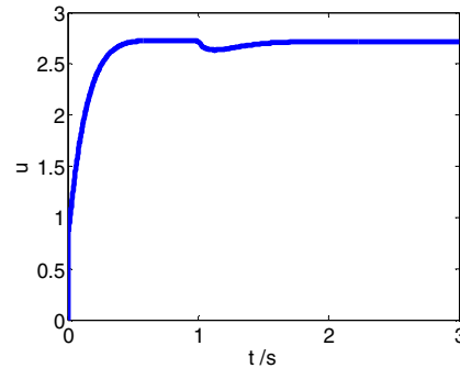
Fig. 5(b). Fuel flow response curve
