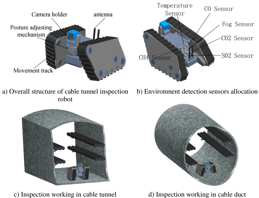
Fig. 1. The small track cable inspection robot
