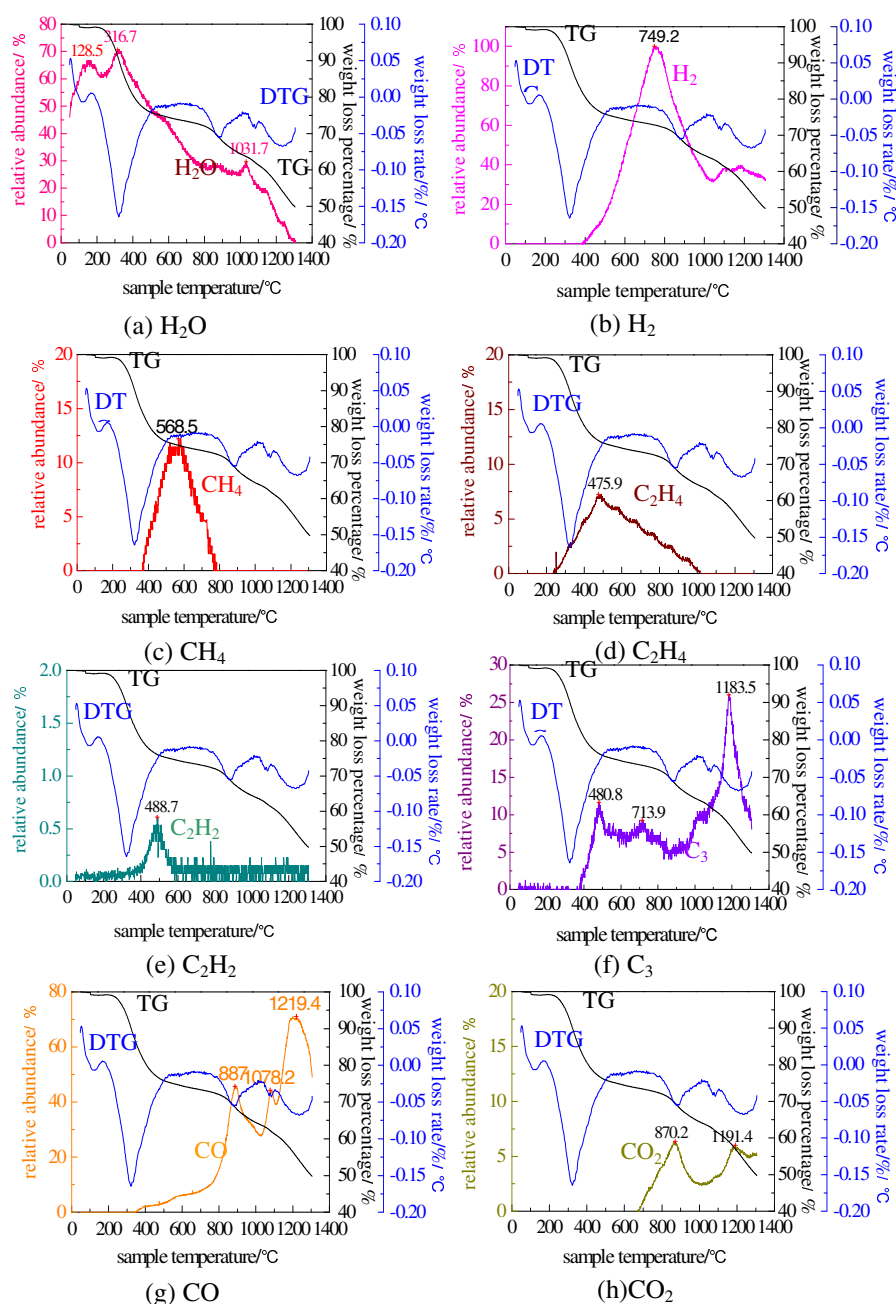
Fig. 2. The TG-MS curves of coal tar during the pyrolysis
