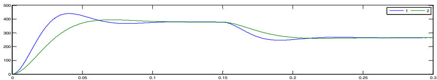
Fig. 7. \overline{v_p} waves with and without state feedback
