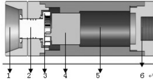
Fig. 2. The structure of intelligent logging unblocking device
