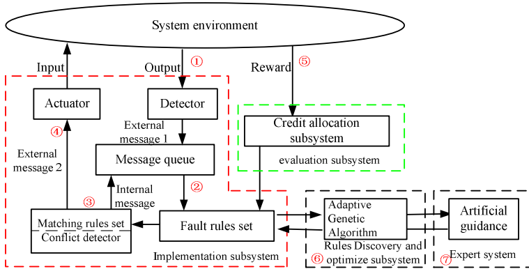
Fig. 2. Fault Rules Intelligence Learning Model Based on Adaptive Genetic Algorithm
