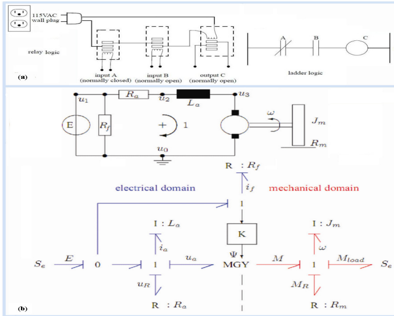
Fig. 1. A) A relay controller and PLC controller. B) Circuit schematics of a motor and bond graph modeling.
