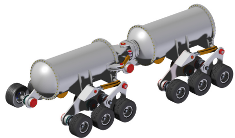
Fig. 1. Structure of composite wheeled submarine walking mechanism
