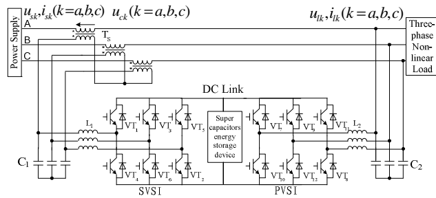
Fig. 1. The structure of UPQC based on super capacitor storage system
