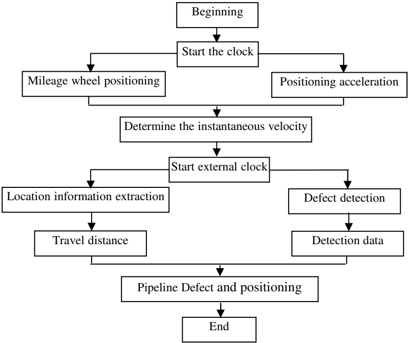
Fig. 4. The structure and localization process Detection equipment
