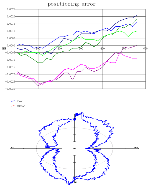
Fig. 6. Experimental results of position errors and rotary errors
