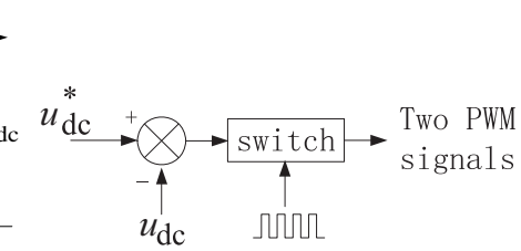
Fig. 6. Control strategy for the energy storage unit at the DC side
