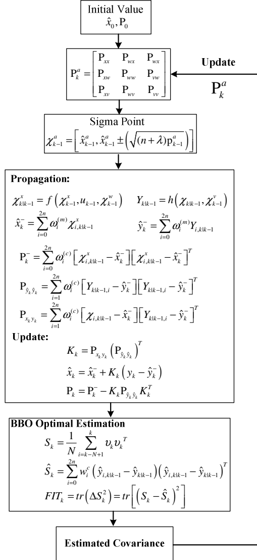
Fig. 4. Flow chart for BBO-UKF Algorithm
