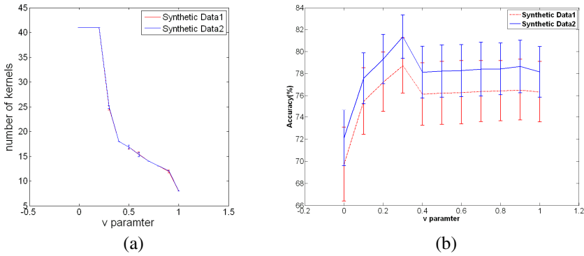
Fig. 2. The number of learned kernel and the accuracy of our algorithm on the synthetic data1 and the synthetic data2. (a). the number of kernels. (b). the accuracy. The best accuracy for all datasets is achieved while v=0.3 . The number of learned kernels will decrease when v increase.
