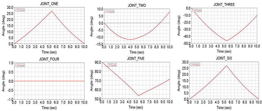
Fig. 3. Six curves of each joint angle in ADAMS
