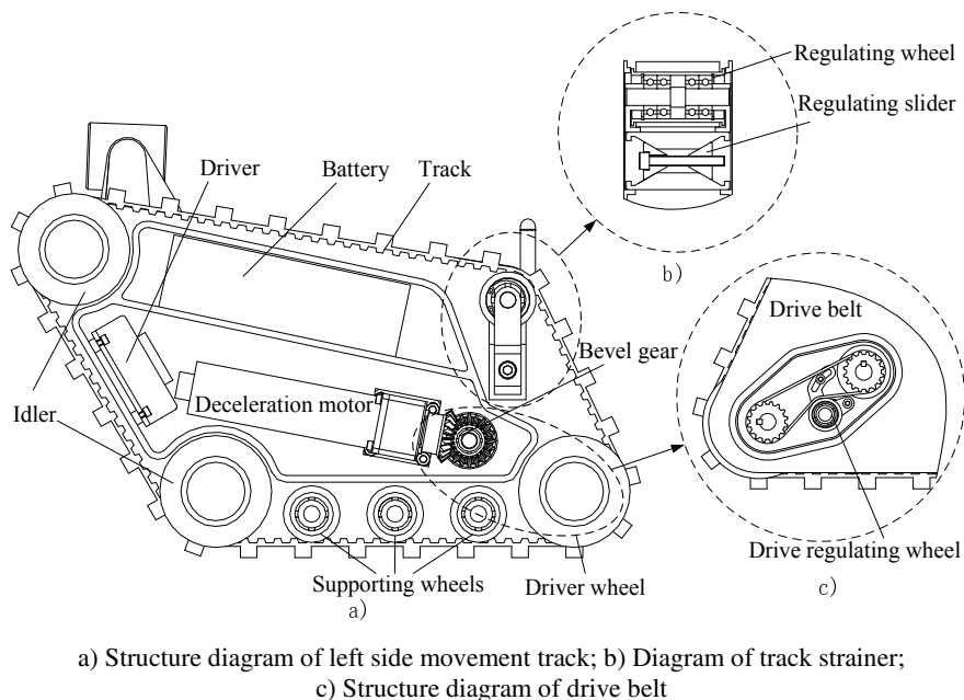
Fig. 2. The schematic of left side track movement mechanism
