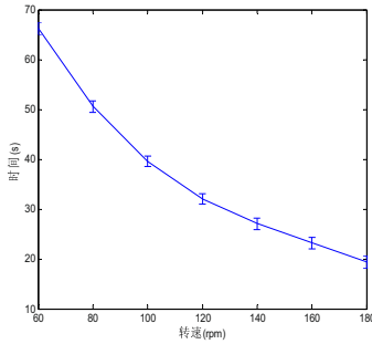
Fig. 3. The motor speed and the running time curve
