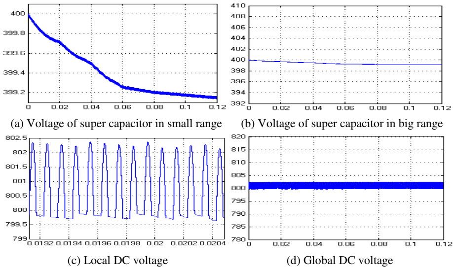
Fig. 7. Simulation results
