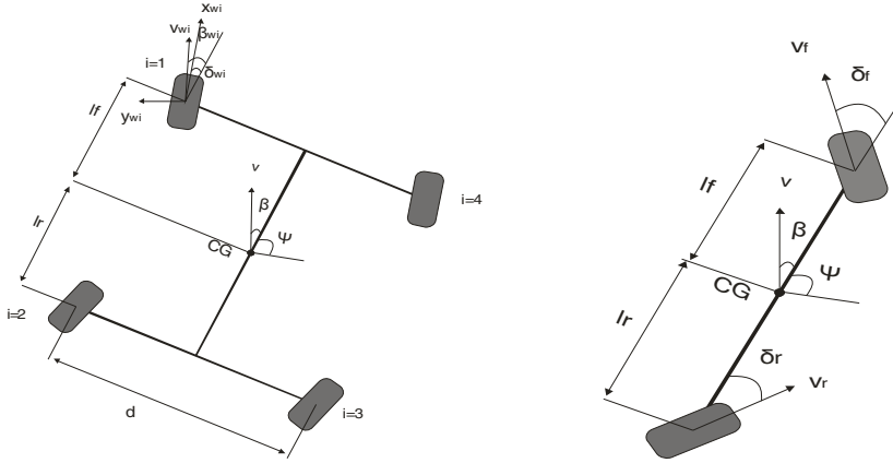
Fig. 1. Kinematics of the four driving/steering wheels Fig. 2. Kinematic model of a bicycle
