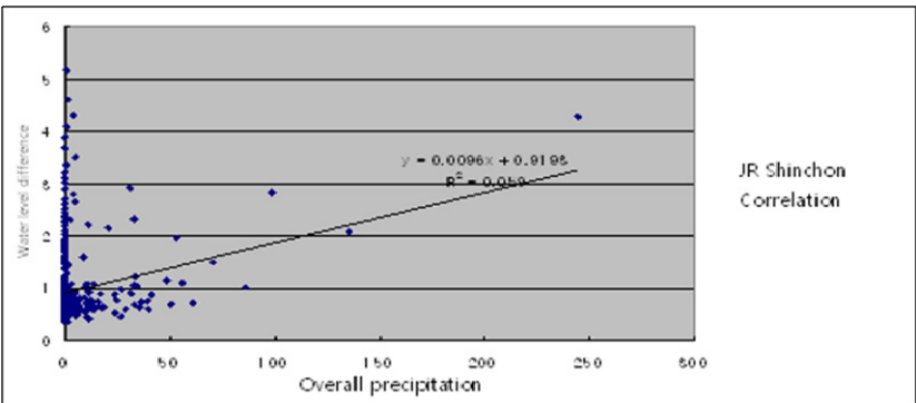
Fig. 7. Association analysis 2
