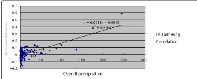
Fig. 8. Association analysis 3
