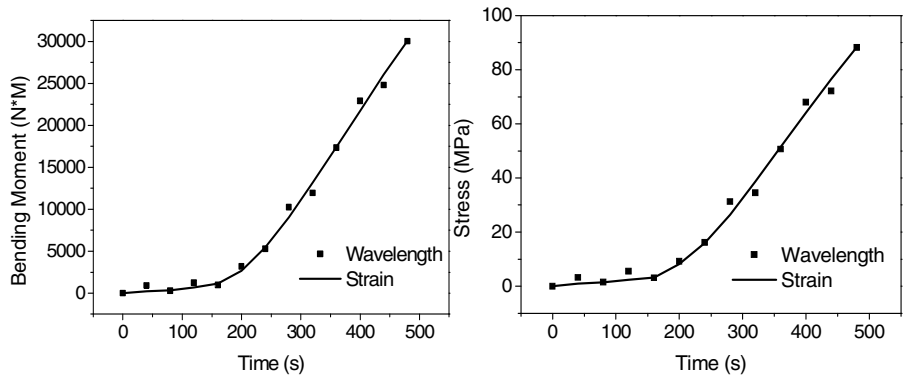
Fig. 5. Graphic measured values of bending moment and stress
