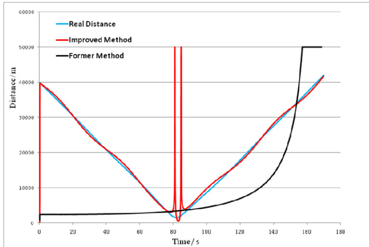
Fig. 3. Simulation results
