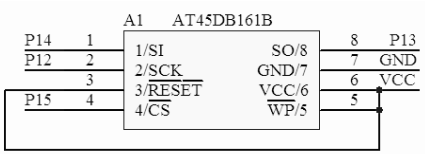
Fig. 7. Data storage circuit
