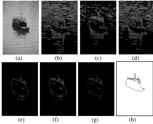
Fig. 2. Information images by QFDD, Canny, Sobel, LOG. (a)original, (b)Canny, (c) Sobel, (d)LOG, (e) v=1.2 QFDD, (f) v=1.5 QFDD, (g) v=1.9 QFDD, (h) Human.
