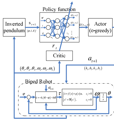
Fig. 3. Biped robot RL control system
