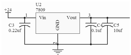
Fig. 6. 7809 circuit connection diagram
