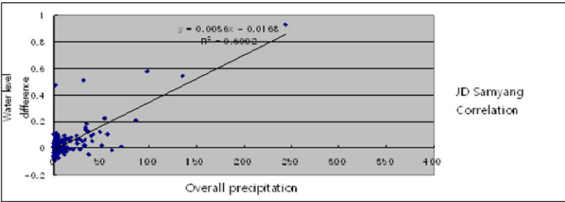
Fig. 6. Association analysis 1
