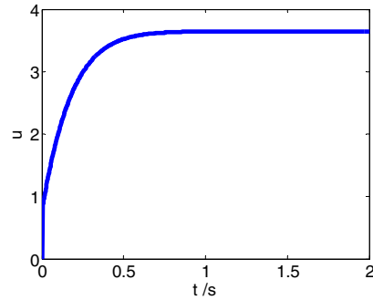
Fig. 4(b). Fuel flow response curve
