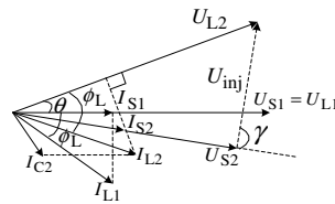
Fig. 3. Vector diagram of UPQC
