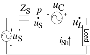
Fig. 2. Equivalent circuit
