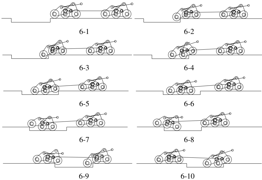
Fig. 6. Adaptive terrain the obstacle-surmounting course sports diagram
